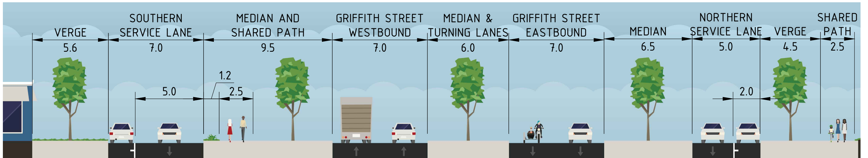
TYPICAL SECTION - GRIFFITH STREET, MADDINGLEY (LOOKING WEST FROM OSBORNE STREET)
