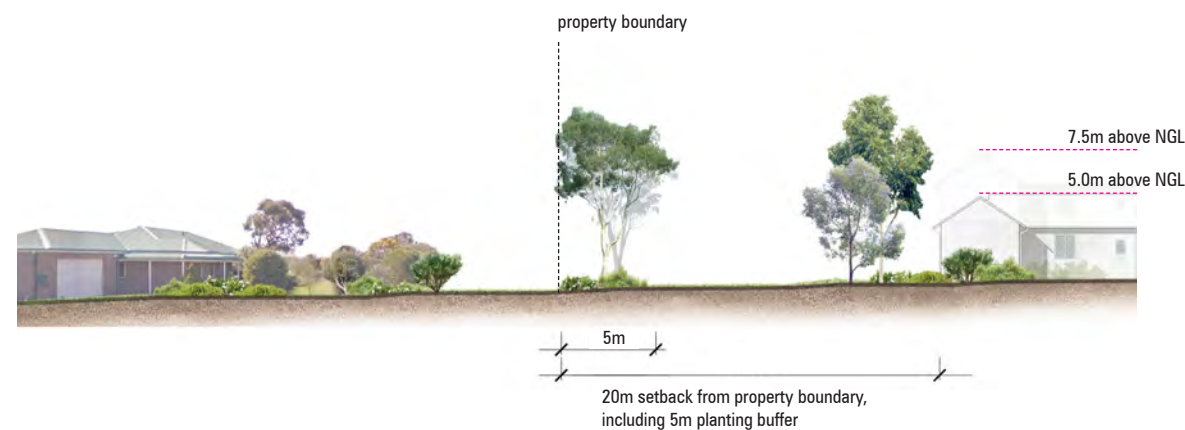
Section E-E (southern boundary interface with rear fence of existing housing) 1:200 @ A1
